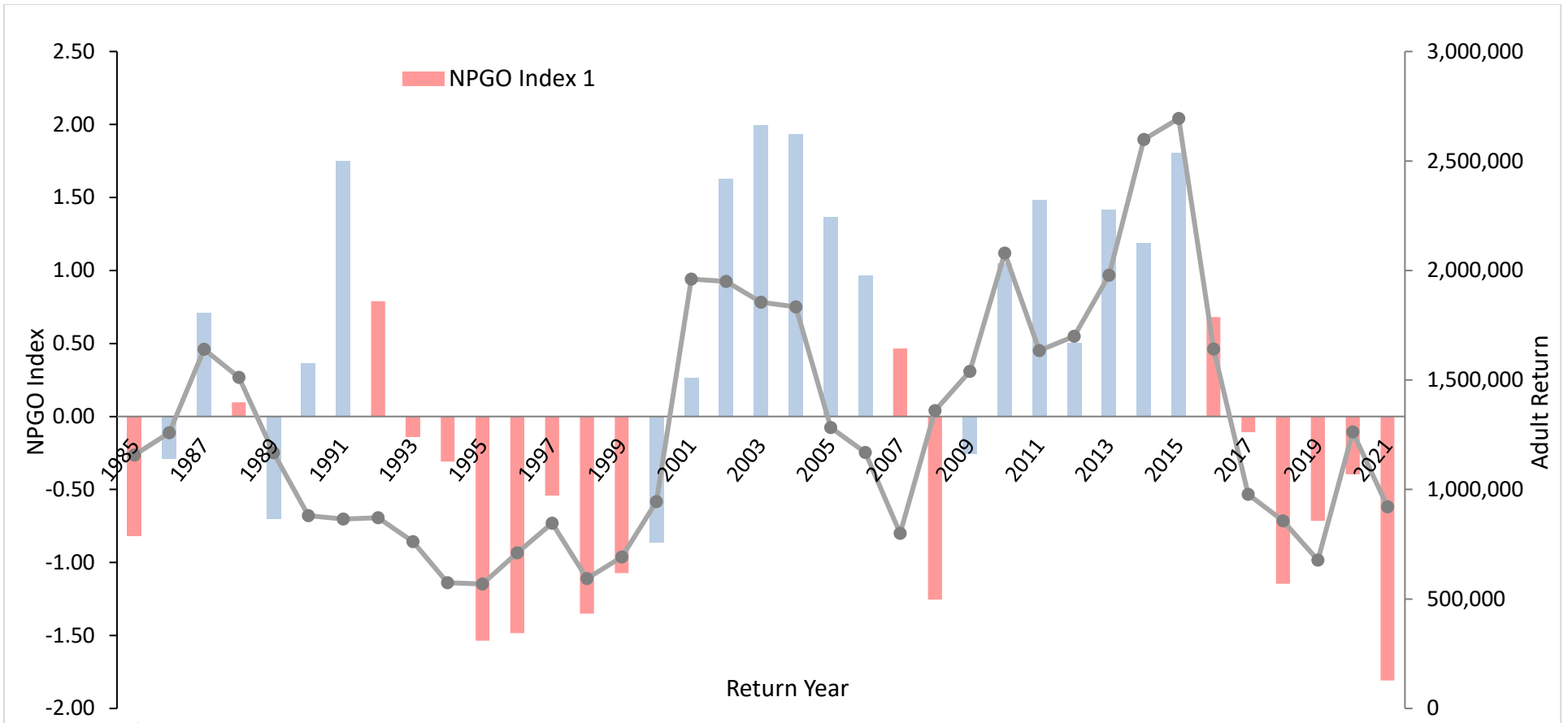
Figure X. Annual return of adult salmonids to the Columbia River mouth and corresponding NPGO Index, 1985–2021. Positive (blue) NPGO (cool) ocean conditions and negative (red) NPGO represents relatively poor (warm) ocean conditions.
